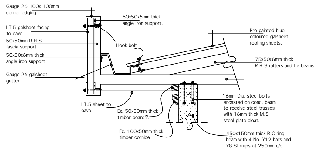
EAVE DETAIL
